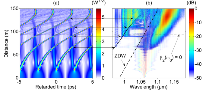
FIG. 2. Temporal (a) and spectral (b) evolutions of a dual-pump input inside a DDF. (a) Square root of the intensity on a linear scale in \sqrt{W} . (b) Normalized spectral intensity in decibels. The two pumps are separated in frequency by 400 GHz and their total power is 1 W. The dashed black line shows the distance at which \beta_2 = 0 at the pumps' center wavelength. Double arrows mark locations of temporal reflections in (a) together with the corresponding wavelengths in (b). The solid black line in (b) shows the theoretical prediction of the temporal reflection model discussed in the text. The dashed line shows the zero-dispersion wavelength.
