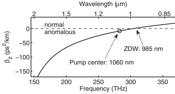
FIG. 1. Dispersion parameter \beta_2 at the input end of the fiber. The circle denotes \nu_0 . The zero-dispersion wavelength of the PCF is 985 nm.
