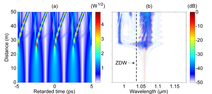
FIG. 4. Temporal (a) and spectral (b) evolutions under conditions identical to those in Fig. 3 except that the value of \beta_2 at the pump-center wavelength was changed to -2.684 \text{ ps}^2/\text{km} .
