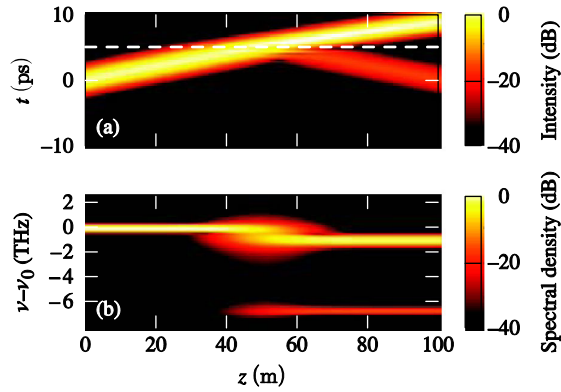
FIG. 1 (color online). Evolution of (a) the pulse shape and (b) the spectrum in the presence of a temporal boundary at T_B = 5 ps (dashed white line) with \beta_B = 0.5 m ^{-1} . Time is measured in a reference frame that is moving with the temporal boundary.
