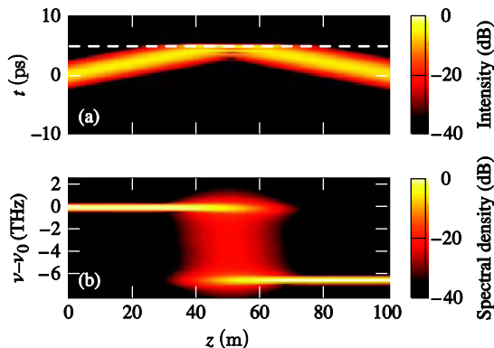
FIG. 3 (color online). (a) Temporal and (b) spectral evolutions of an optical pulse undergoing TIR at a temporal boundary located at T_B = 5 \text{ ps} (dashed white line) with \beta_B = 1.4 \text{ m}^{-1} . Time is measured in a reference frame that is moving with the temporal boundary.
