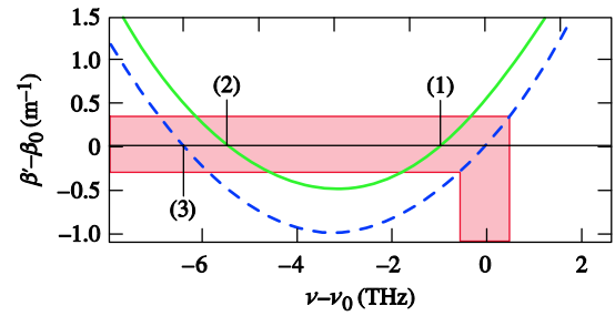
FIG. 2 (color online). Dispersion curves for t < T_B (dashed blue curve) and t > T_B (solid green curve). The shaded region shows the spectral extent of the input pulse and the corresponding range of propagation constants for t < T_B . The slope of the dispersion curve is related to the speed of the pulse relative to the traveling temporal boundary.
