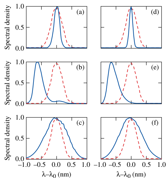
Fig. 5. Comparison of (a)–(c) experimental and (d)–(f) simulated output spectra (solid blue line) for (a), (d) \theta = 0 , (b), (e) \theta = \pi/2 , and (c), (f) \theta = \pi . The input spectrum is shown by the dashed red line.
