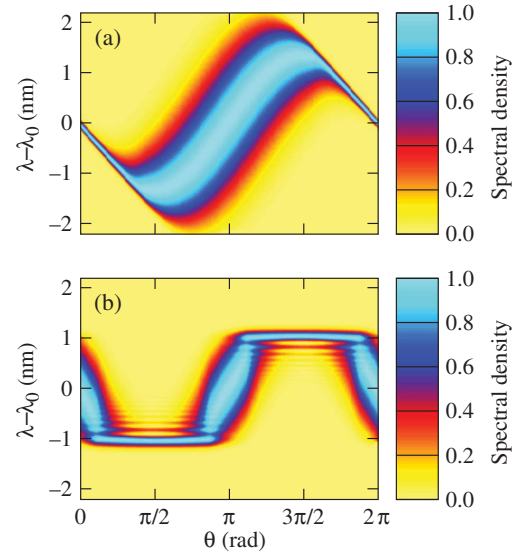
Fig. 1. Surface plots showing simulated output spectra for different values of \theta when (a) 1.5 ps and (b) 20 ps Gaussian pulses are sent through a phase modulator acting as a time lens. The color bars show the range of spectral density, normalized to 1 at its peak for each value of \theta .
