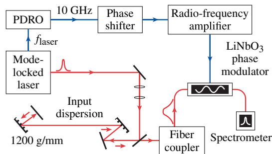
Fig. 3. Experimental setup for a time-to-frequency converter using a phase modulator as a time lens. PDRO: phase-locked dielectric resonator oscillator.
