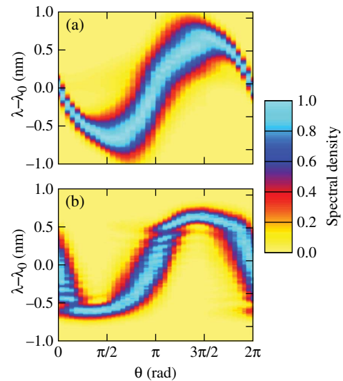
Fig. 4. Surface plots showing experimental output spectra for different values of \theta when input pulses were filtered to produce (a) 0.407- and (b) 0.108-nm-wide input spectra. The color bars show the range of spectral density, normalized to 1 at its peak for each value of \theta .
