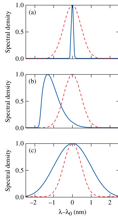
Fig. 2. Comparison of input (dashed) and output (solid) spectra for a 1.5 ps input pulse at clock phases (a) \theta = 0 , (b) \theta = \pi/2 , and (c) \theta = \pi .
