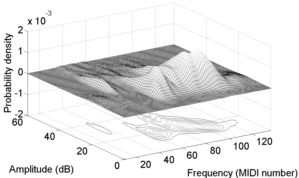
Fig. 2. Illustration of the probability density of p(f_k, a_k | s_k = 1) , which is calculated from the spurious peaks of the polyphonic training data. The contours of the density is plotted at the bottom of the figure.
