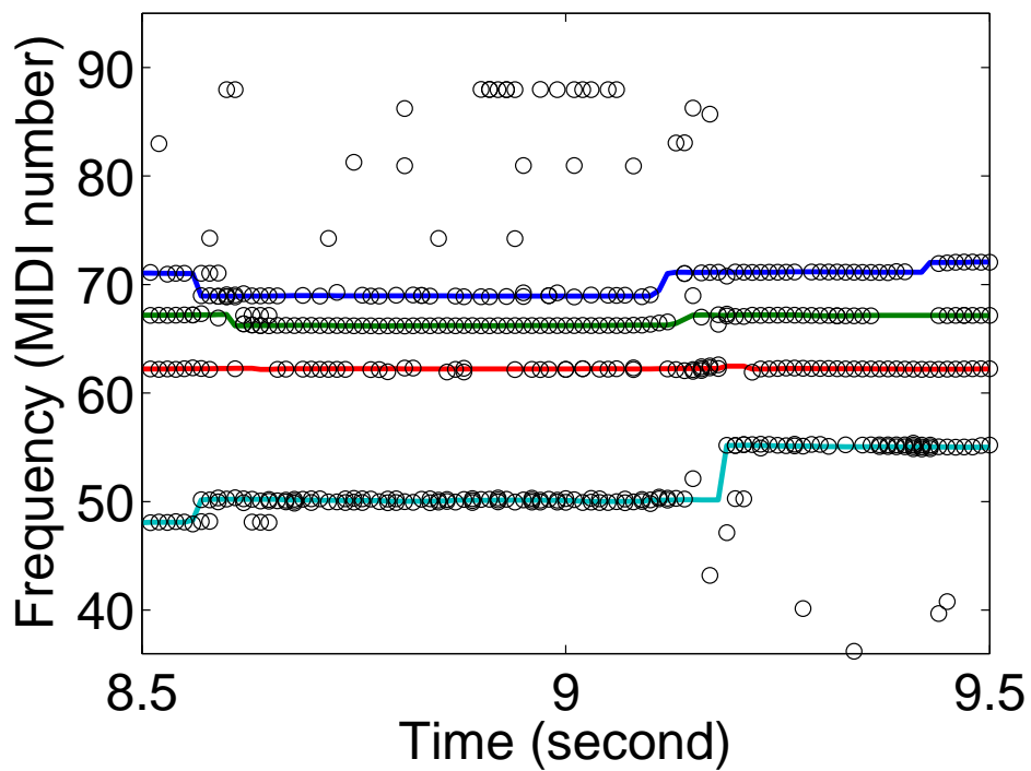
(a) Before refinement
