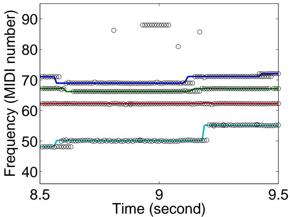
(b) After refinement
