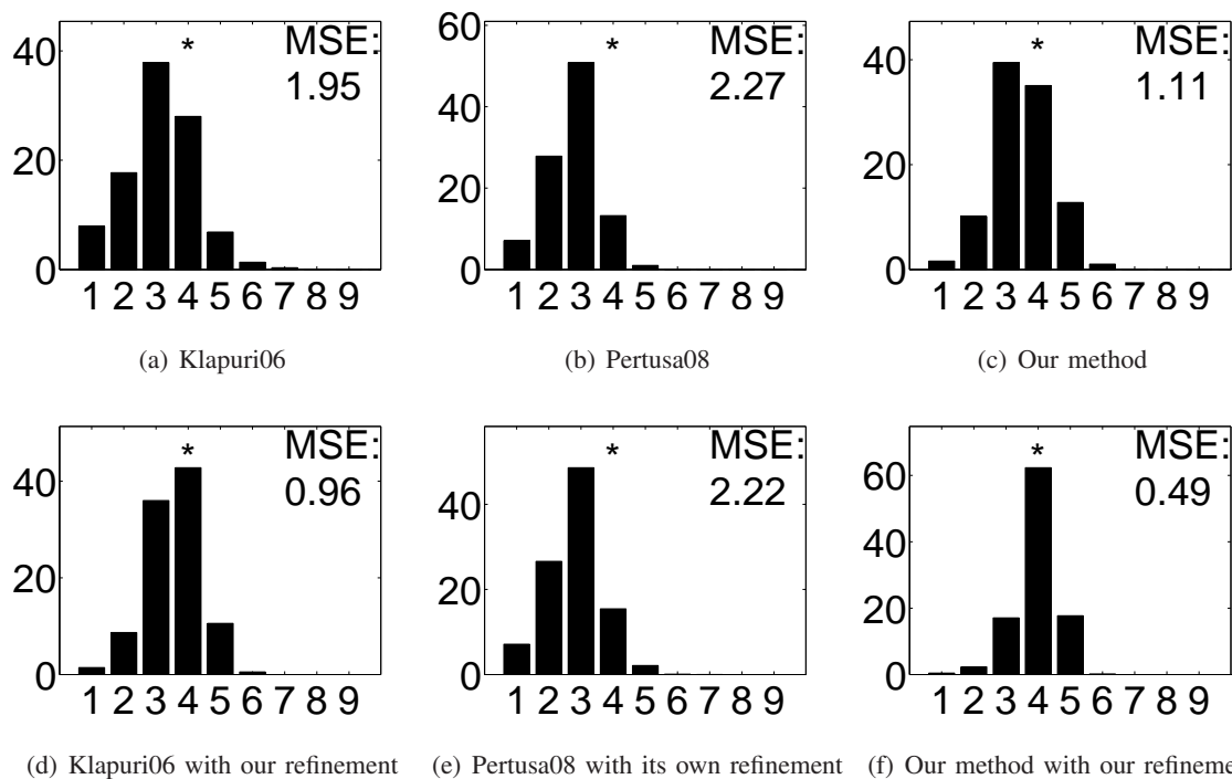
Fig. 7. Polyphony estimate histogram on the total 33,000 frames of the testing music pieces. X-axes represent polyphony. Y-axes represent the proportion of frames (%). The asterisk indicates the true polyphony.
